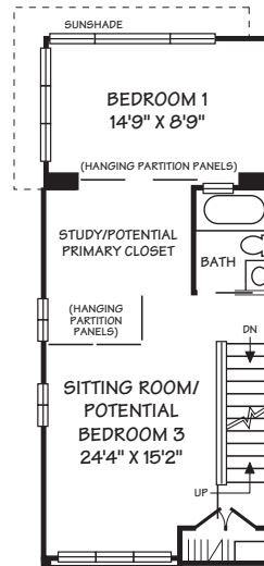
THIRD LEVEL 8'1" CEILING
